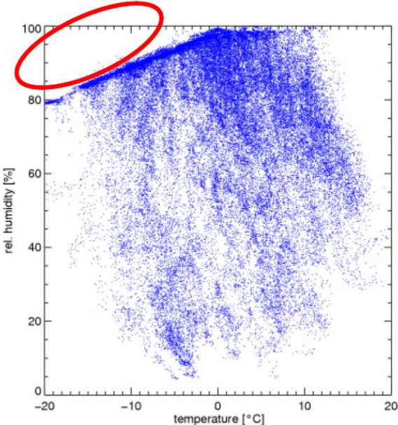
Figure 4-4: Relative humidity measured according WMO/CIMO standards does not reach saturation anymore at temperatures below 0°C (red area).
